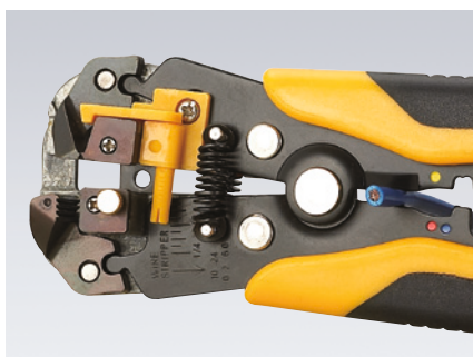
Cutting(0.25-6.0mm 2 )
