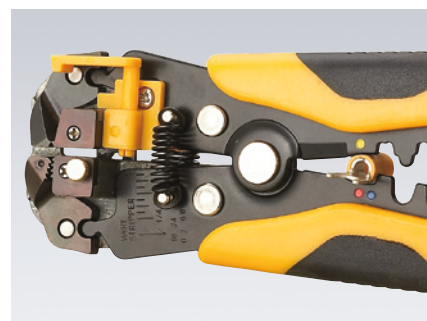
Crimping terminal (0.5-6.0mm 2 )
